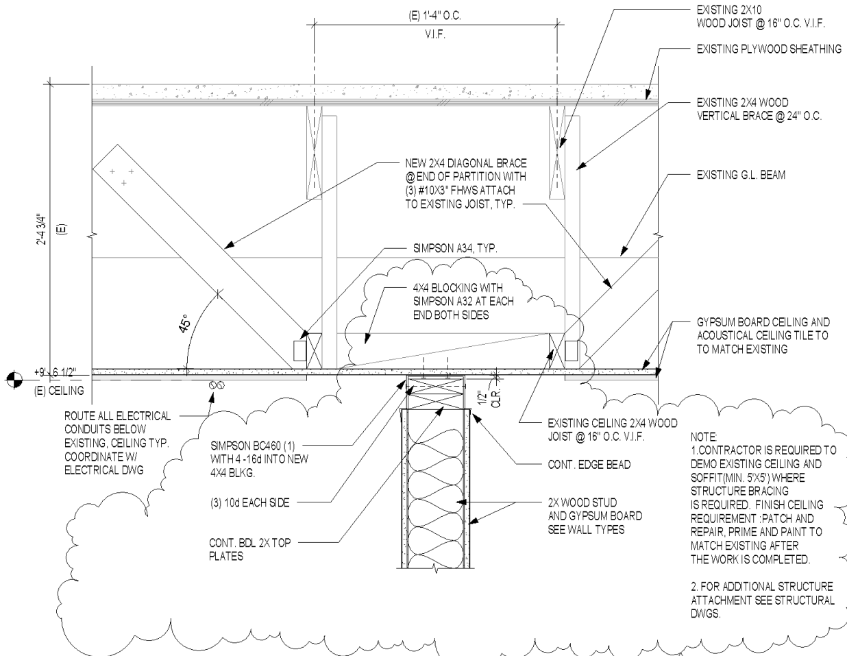
2 WALL HEAD / DIAGONAL BRACE DTL @ EXISTING CEILING JOIST 1 1/2" = 1'-0"
